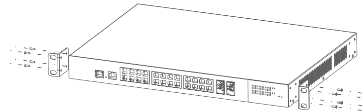
Figure 2-1 Install hangers diagram
