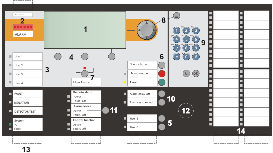
Indication and operating elements
