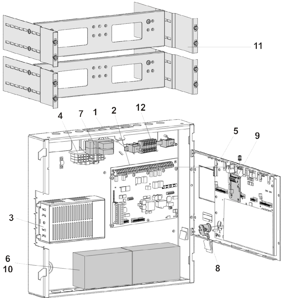
Layout of FC721
